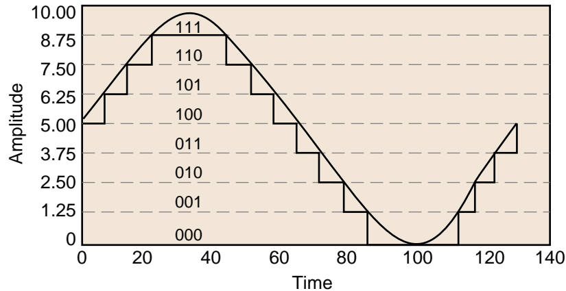
Figure 3. Digitized Sine Wave with a Resolution of Three Bits
