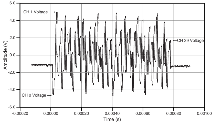
Figure 5. The input to an instrumentation amplifier that is multiplexing 40 DC signals appears to be a high-frequency AC signal.
