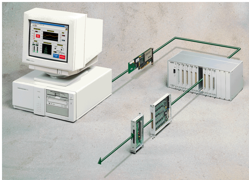
Figure 2. The SCXI Signal Conditioning Front-End System for Plug-In DAQ Boards
