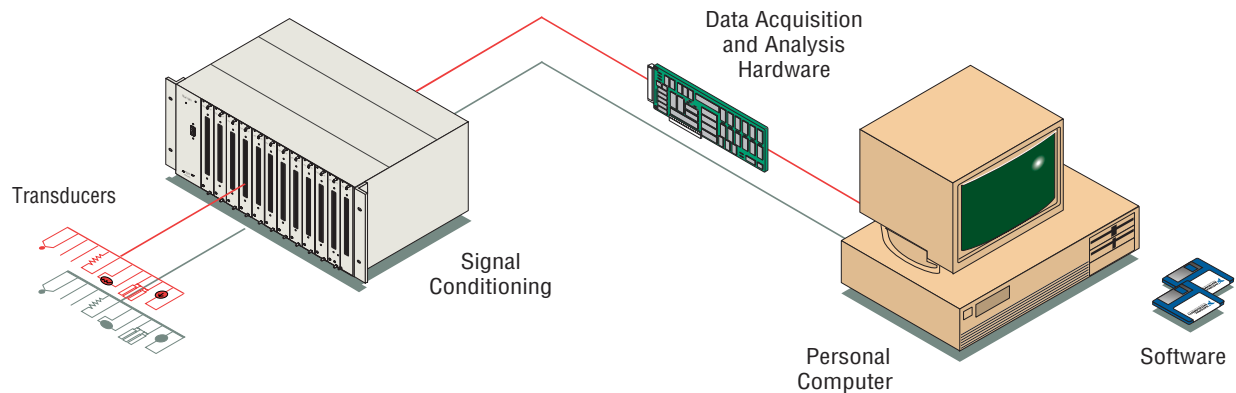
Figure 1. The Typical PC-Based DAQ System
