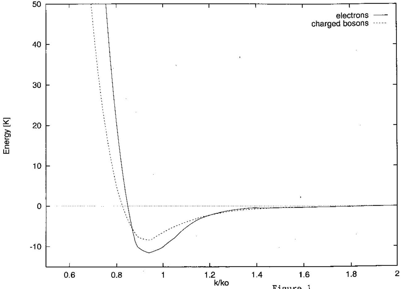
Effective pair potential nv_{eff}(k) as defined in equation (2) (in Kelvin degrees), plotted against the reduced wave number k for the 3D electron fluid at r_s = 100 (full curve) and for the 3D fluid of charged bosons at r_s = 160 (dashed curve). The wave number is scaled by the length k_0 of the first reciprocal lattice vectors in the respective BCC crystals.
